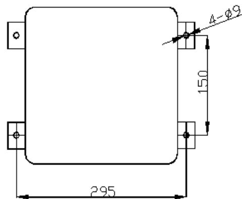
MOUNTING DIMENSIONAL DRAWING
